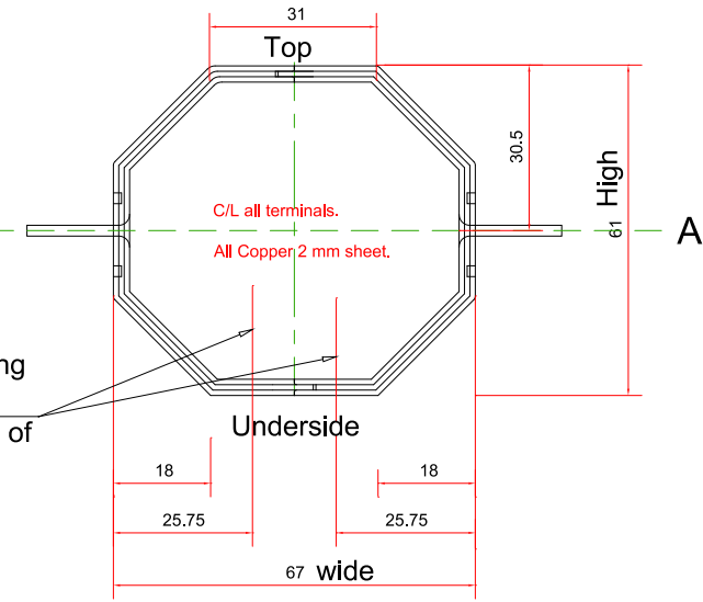
Cross section thru' Nova busbar
